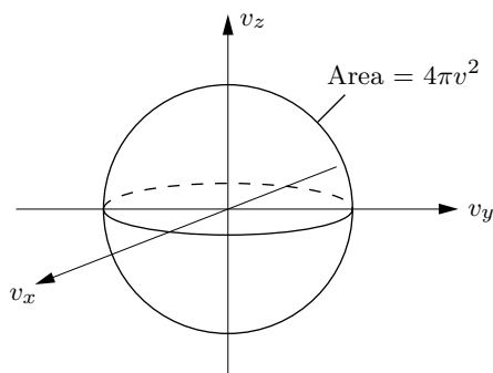
Figure 6.12. In “velocity space” each point represents a possible velocity vector. The set of all vectors for a given speed v lies on the surface of a sphere with radius v .
