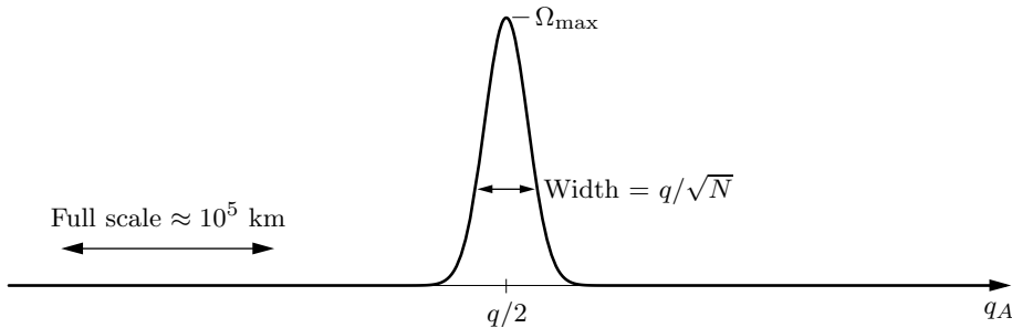
Figure 2.7. Multiplicity of a system of two large Einstein solids with many energy units per oscillator (high-temperature limit). Only a tiny fraction of the full horizontal scale is shown.
