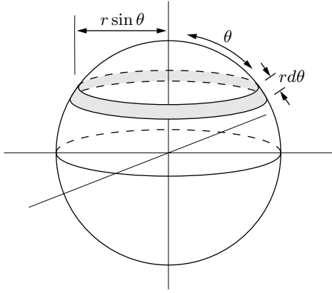
Figure B.6. To calculate the area of a sphere, divide it into loops and integrate. To calculate the area of a hypersphere , do the same thing.
