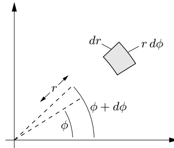
Figure B.2. In polar coordinates, the infinitesimal area element is (dr)(r d\phi) .
