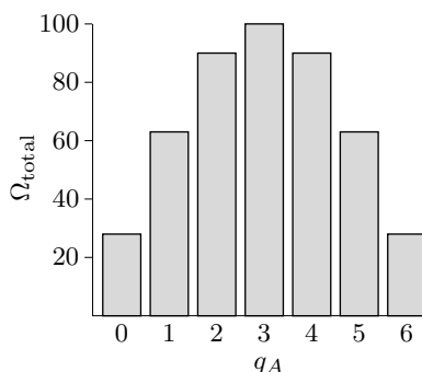
Figure 2.4. Macrostates and multiplicities of a system of two Einstein solids, each containing three oscillators, sharing a total of six units of energy.
