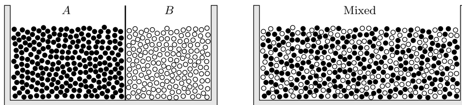
Figure 5.24. A collection of two types of molecules, before and after mixing.
