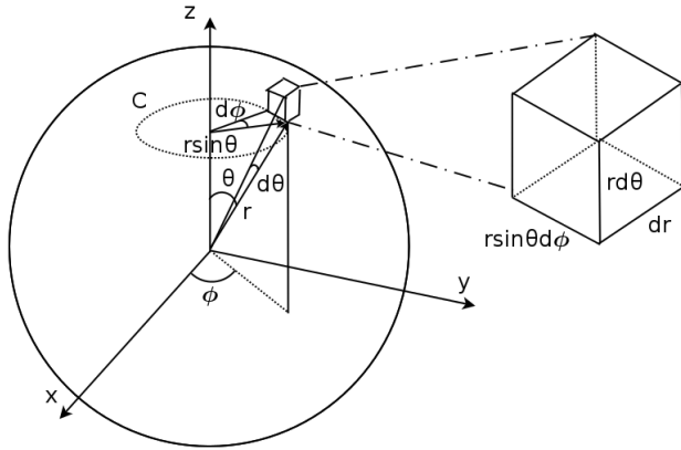
Figure 2.16: Spherical coordinates
