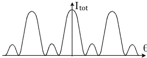
Figure 14.12: Intensity graph
