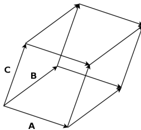
Figure 3.8: Triple product
