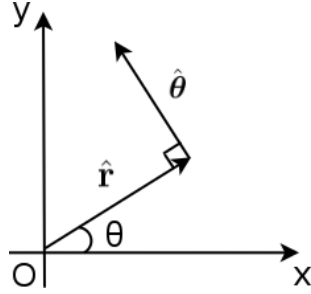
Figure 4.7: Polar coordinates
