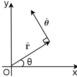
Figure 2.6: Polar coordinates
