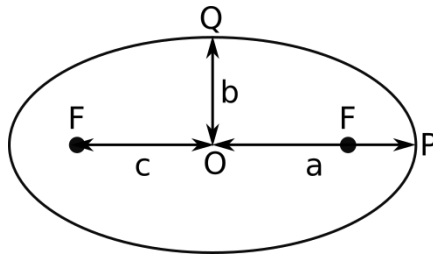
Figure 8.1: Ellipse
