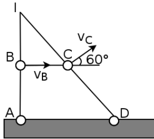
Figure 3.19: ICoR of rod BC
