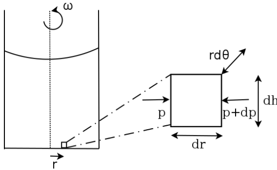
Figure 9.5: Rotating fluid
