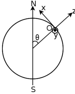
Figure 11.5: Coordinate system at colatitude \theta
