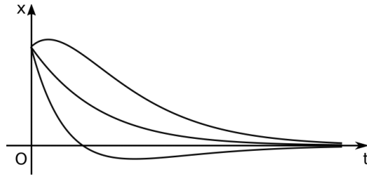
Figure 10.8: Critical damping
