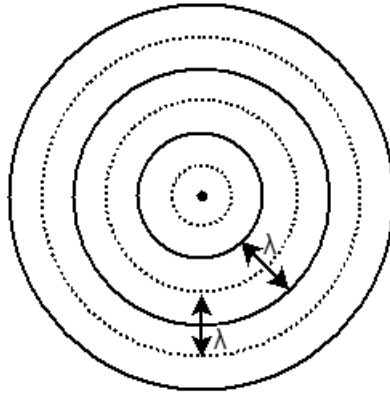
Figure 13.5: Ripples
