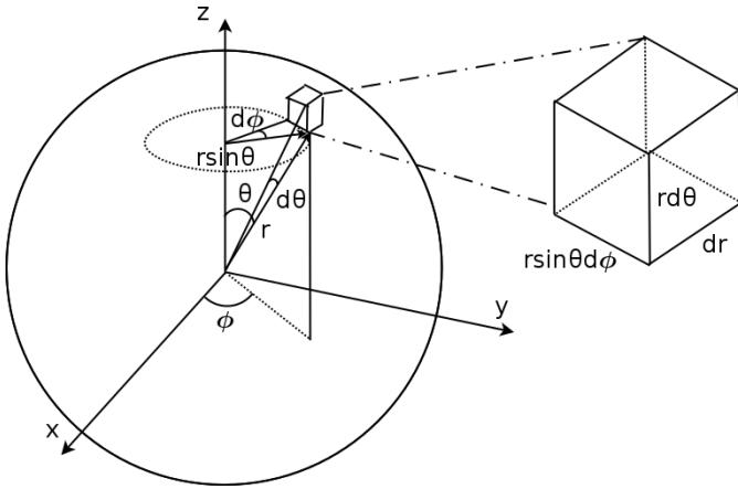
Figure 5.5: Spherical coordinates
