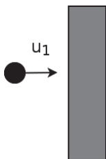
Figure 6.7: Collision of gas particle with massive wall
