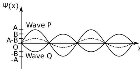
Figure 14.6: Destructive interference
