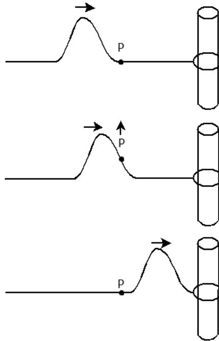
Figure 13.1: Traveling pulse
