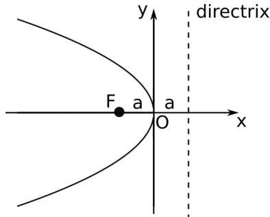
Figure 8.2: Parabola
