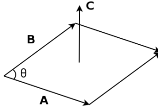
Figure 3.7: Cross product
