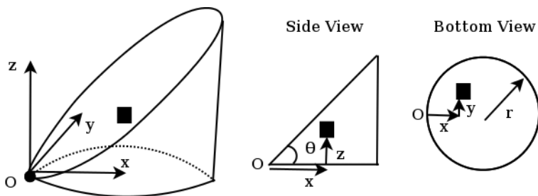
Figure 4.30: Cylindrical segment
