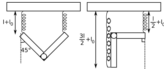
Figure 7.34: Static equilibrium positions
