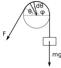
Figure 7.24: Holding a weight around a rough pole
