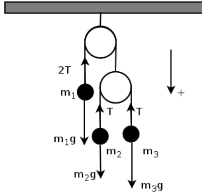
Figure 4.16: Atwood's machine 2
