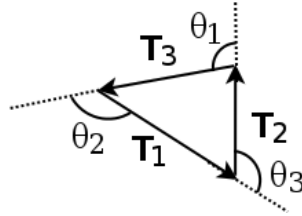
Figure 4.24: Force triangle
