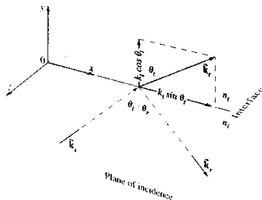
Figure 4.54 Propagation vectors for internal reflection.
