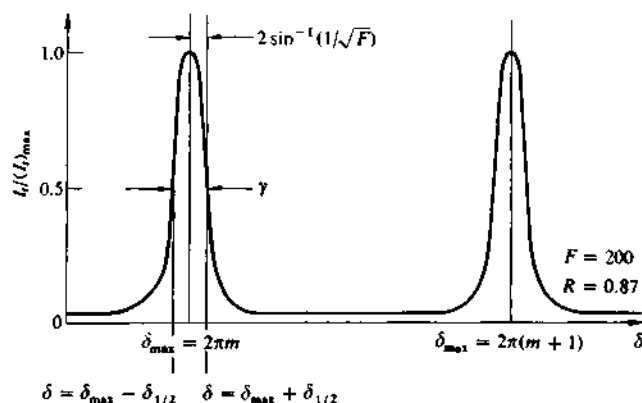
Figure 9.45 Fabry–Perot fringes.
