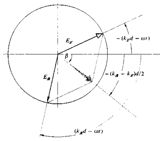
Figure 8.51 The superposition of an \mathcal{R} - and an \mathcal{L} -state at z = d ( k_{\mathcal{L}} > k_{\mathcal{R}} , \lambda_{\mathcal{L}} < \lambda_{\mathcal{R}} , and \nu_{\mathcal{L}} < \nu_{\mathcal{R}} ).
