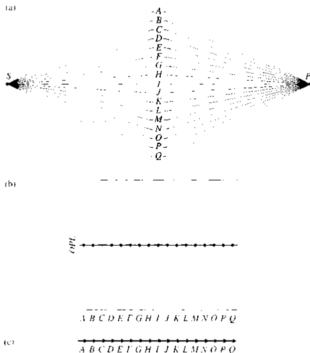
Figure 5.32 Feynman's analysis of the thin lens via QED. (a) A number of possible paths from S to P . (b) The OPL for light along each path. (c) The corresponding probability-amplitude phasors all adding in-phase.
