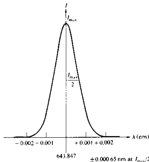
Figure 7.36 The cadmium red ( \bar{\lambda} = 643.847 nm) spectral line from low-pressure lamp.
