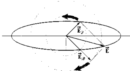
Figure 8.8 Elliptical light as the superposition of an \mathcal{R} - and \mathcal{L} -state.
