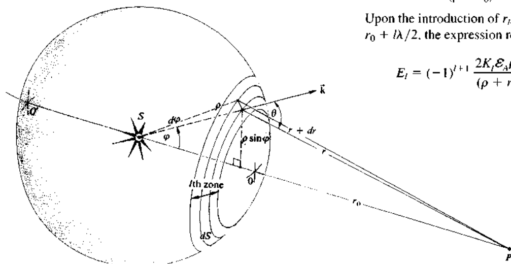
Figure 10.38 Propagation of a spherical wavefront.
