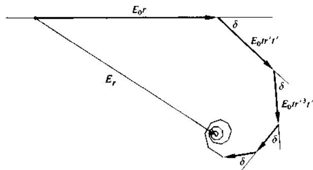
Figure 9.40 Phasor diagram.
