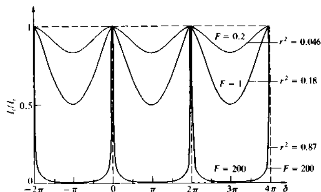
Figure 9.41 Airy function.
