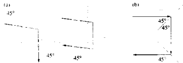
Figure 4.52 Total internal reflection.
