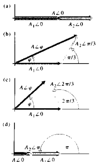
Figure 2.18 The addition of phasors representing two waves having amplitudes of A_1 = 1.0 , and A_2 = 0.9 with four different relative phases, as shown in Fig. 2.14.
