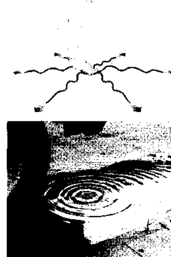
Figure 2.12 Circular waves. (Photo by E.H.)
