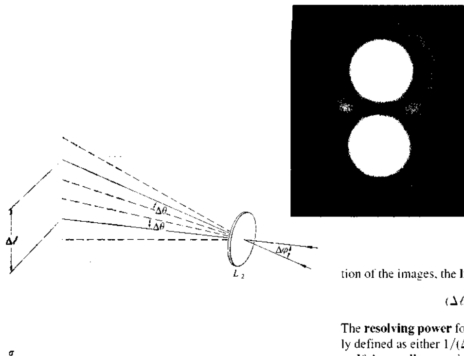
Figure 10.24 Overlapping images.
