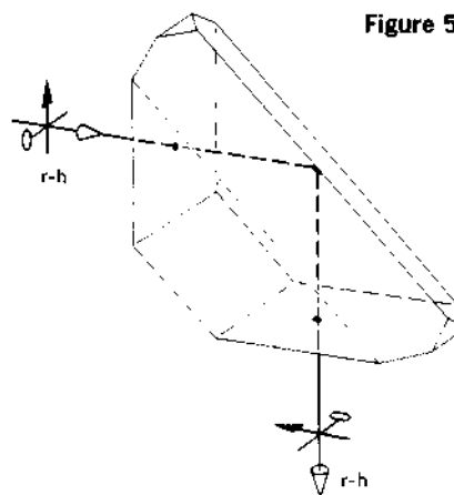
Figure 5.64 The Amici prism.
