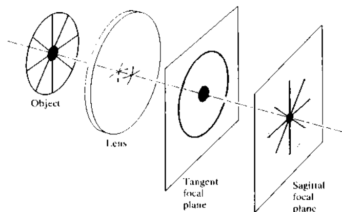
Figure 6.28 Images in the tangential and sagittal focal planes.
