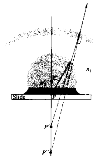
Figure 6.18 An oil-immersion microscope objective.
