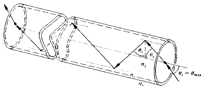
Figure 5.71 Rays in a clad optical fiber.
