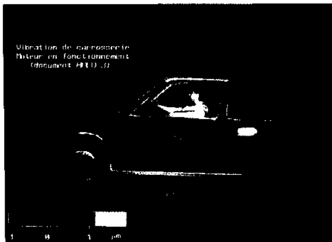
A standing-wave pattern on the side of a car due to vibrations caused by its running engine. The scale is in microns, where 1 \mu\text{m} = 10^{-6} \text{ m} . The photo was made using a holographic technique. (Photo courtesy HOLO3/FTPO.)
