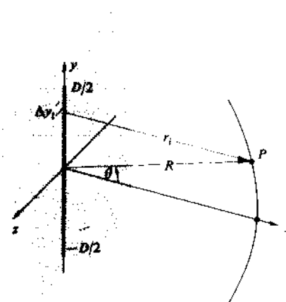
Figure 10.5 A coherent line source.
