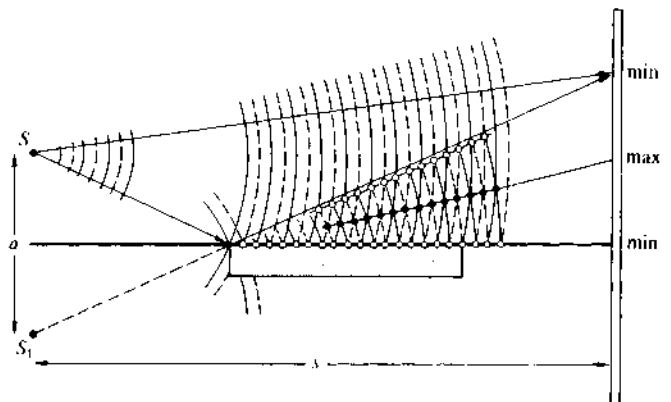
Figure 9.14 Lloyd's mirror.
