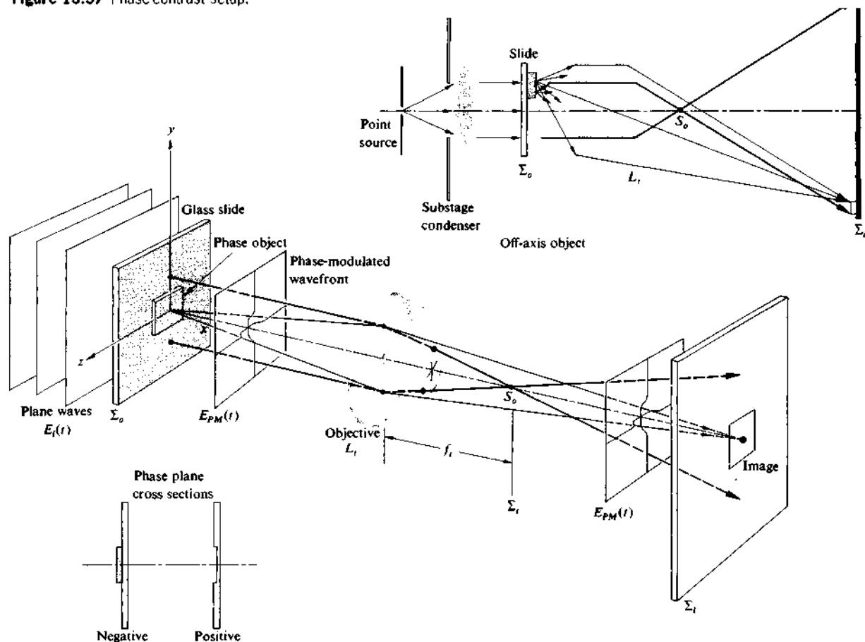
Figure 13.37 Phase-contrast setup.
