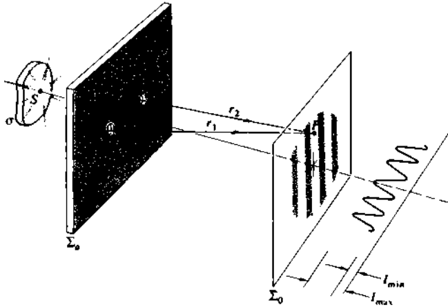
Figure 12.11 Young's Experiment.
