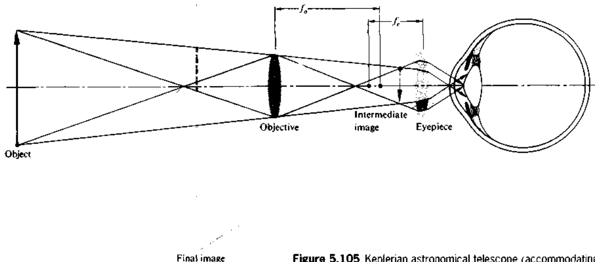
Figure 5.105 Keplerian astronomical telescope (accommodating eye).
