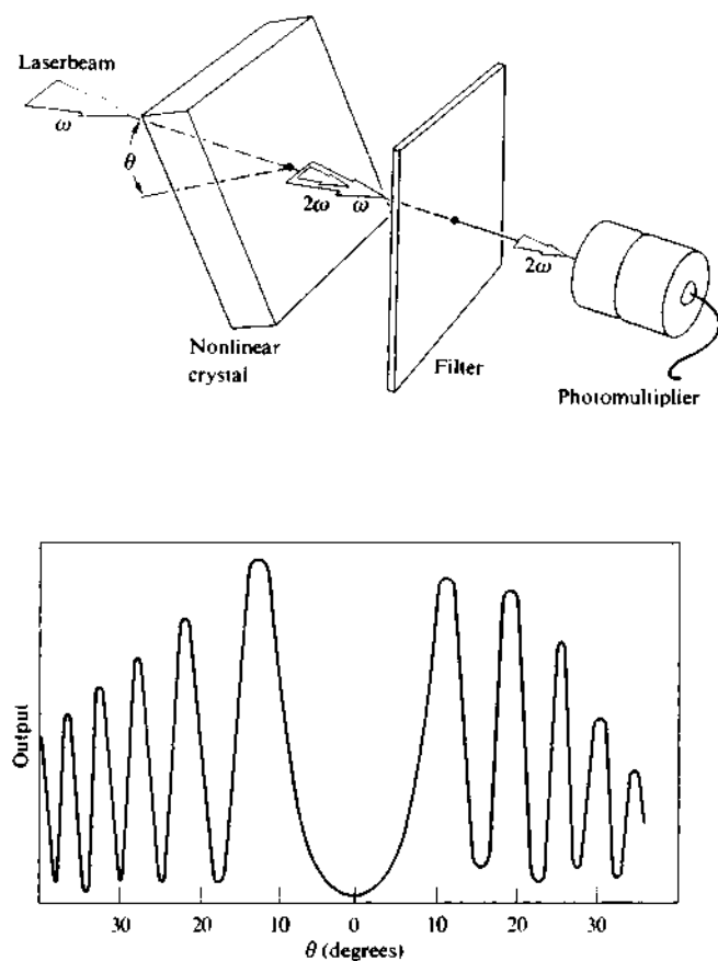
Figure 13.56 Second-harmonic generation as a function of \theta for a 0.78-mm thick quartz plate. Peaks occur when the effective thickness is an even multiple of \lambda_c . [From P. D. Maker, R. W. Terhune, M. Nisenoff, and C. M. Savage, Phys. Rev. Letters 8 , 21 (1962).]
