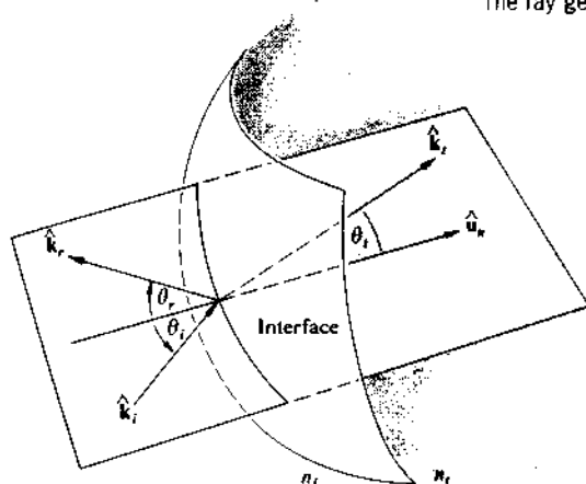
Figure 4.24 The ray geometry.
