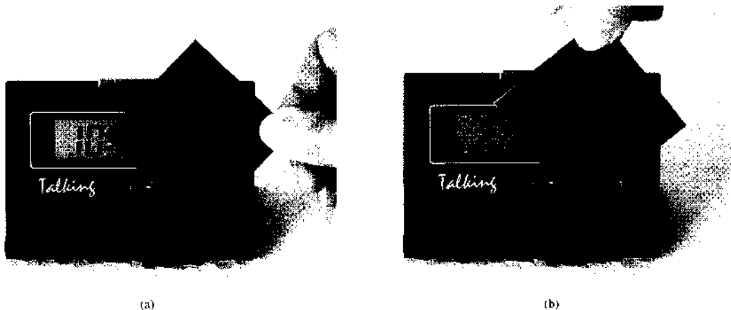
Figure 8.61 (a) A twisted nematic cell between crossed linear polarizers. Light polarized vertically emerges from the device. (b) When a voltage is applied across the cell it no longer rotates the plane of polarization; light polarized horizontally enters and leaves the LC cell. That light is subsequently absorbed by the second polarizer and no light emerges from the device.
