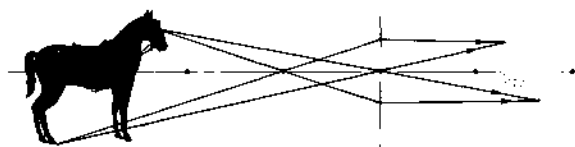
Figure 5.26 The transverse magnification is different from the longitudinal magnification.
