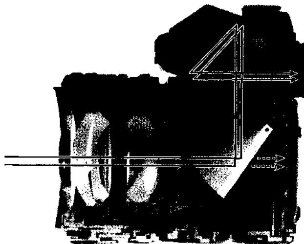
A single-lens reflex camera. Light from the lens hits the mirror and goes up to the prism and out to the eye. When the shutter is released the mirror pops up, the light goes directly to the film, and then the mirror pops back down. (Photo by E.H.)
