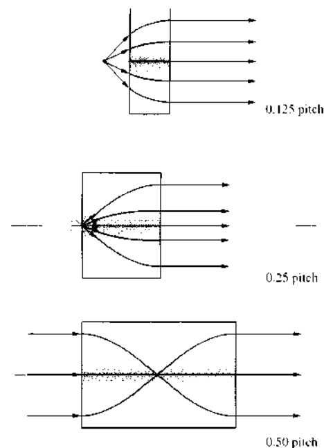
Figure 6.44 Radial GRIN lenses with several pitches used in a few typical ways.
