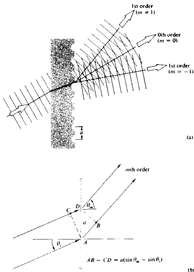
Figure 10.28 A transmission grating.
