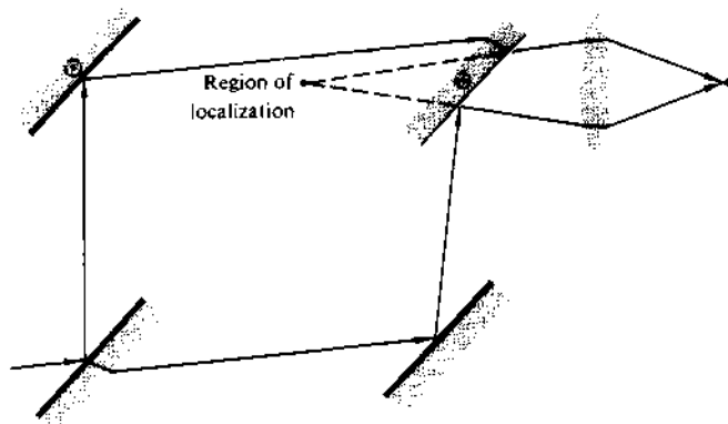
Figure 9.35 Fringes in the Mach-Zehnder Interferometer.
