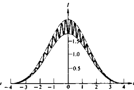
(e) a = 1.7 \text{ cm} \mathcal{V} = |\tilde{\gamma}_{12}| = 0.123, \alpha_{12} = \pi
