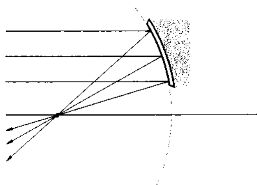
Figure 5.48 An off-axis parabolic mirror element.
