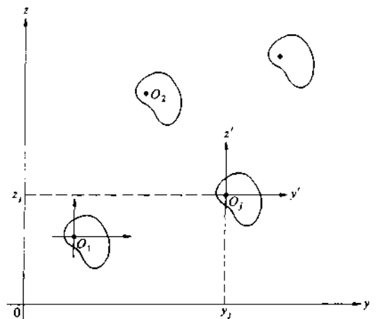
Figure 11.34 Multiple-aperture configuration.
