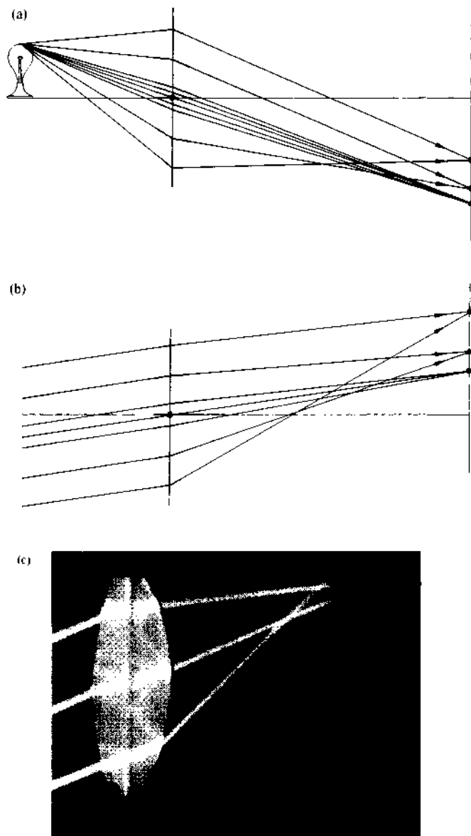
Figure 6.21 (a) Negative coma. (b) and (c) Positive coma. (Photo by E.H.)
