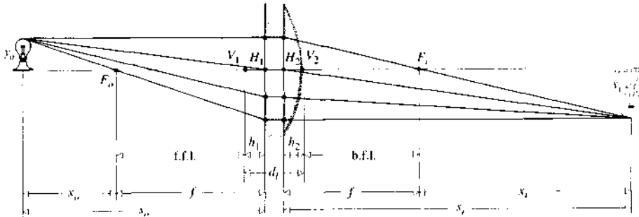
Figure 6.4 Thick-lens geometry.
