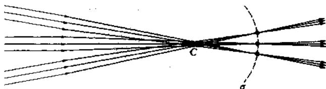
Figure 5.17 Focusing of several ray bundles.
