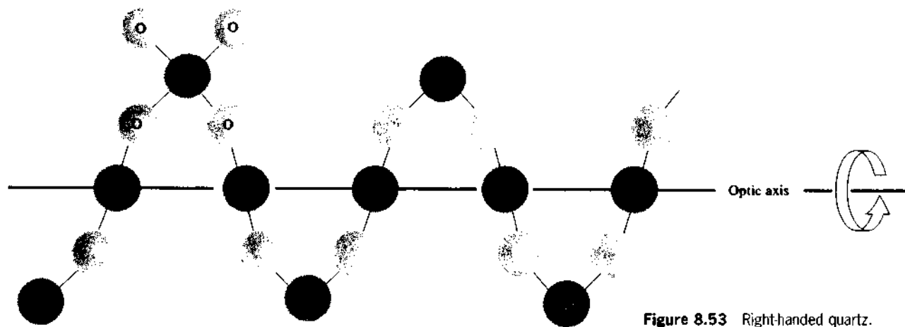
Figure 8.53 Right-handed quartz.
