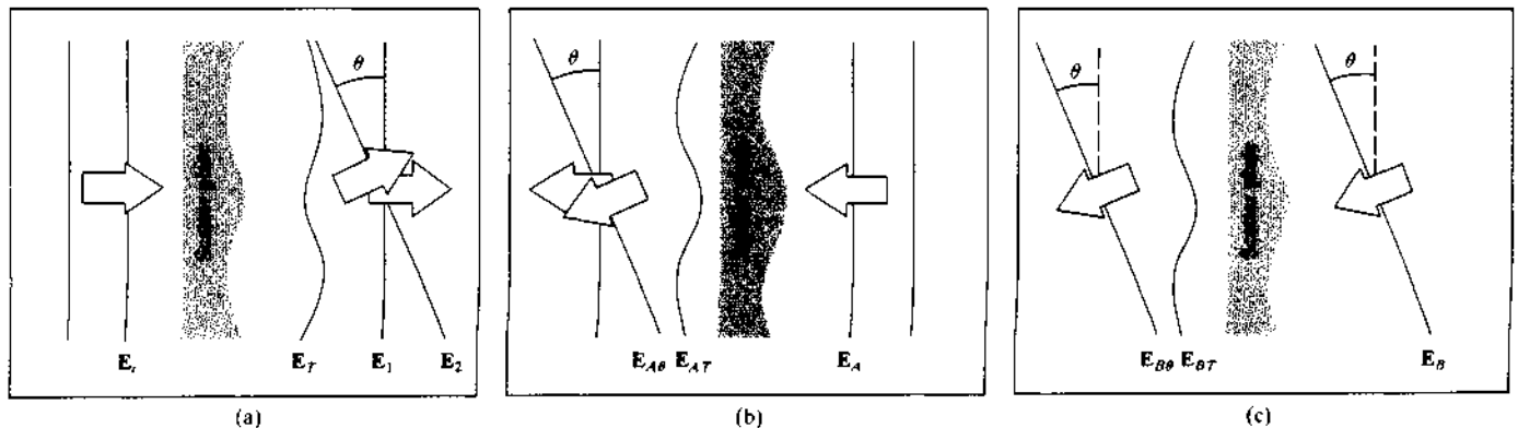
Figure 9.54 Wavefronts passing through the scatter plate.
