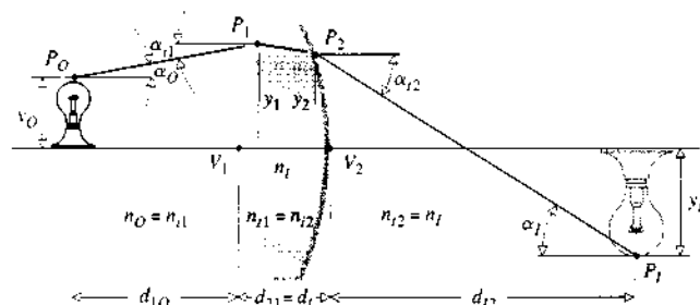
Figure 6.8 Image geometry.
