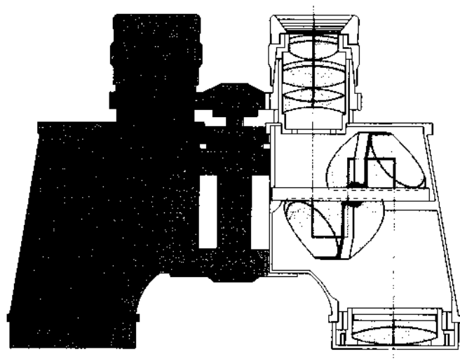
Figure 5.109 A binocular.
