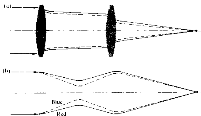
Figure 6.41 Achromatized lenses.
