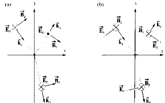
Figure 4.43 Field orientations and phase shifts.
