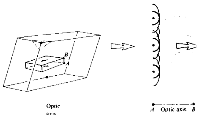
Figure 8.36 A calcite plate cut perpendicular to the optic axis.
