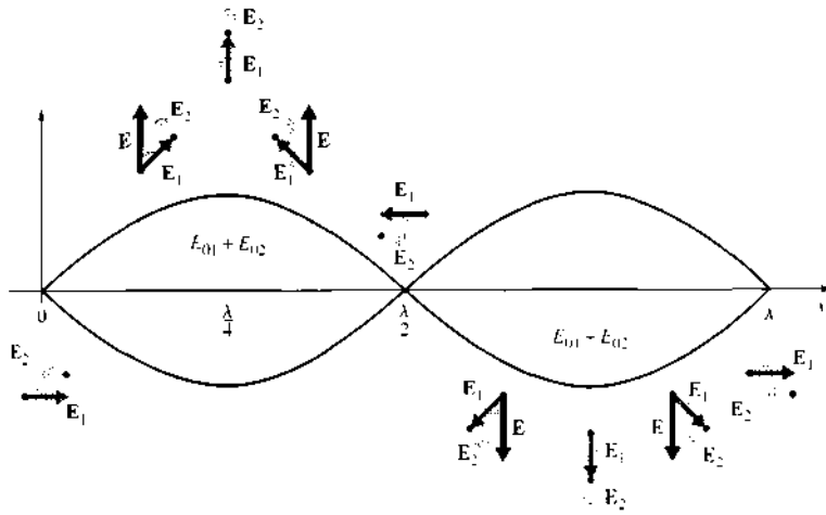
Figure 7.12 The generation of a standing wave from the perspective of phasor addition. The two phasors rotate at the same rate but in opposite directions. Here both waves have the same amplitudes, and that produces complete cancellation at the nodes.
