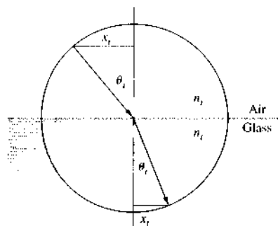
Figure 4.20 Descartes's arrangement for deriving the Law of Refraction.
