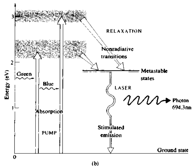
Figure 13.7 Ruby-laser energy levels.
