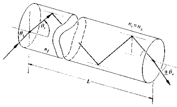
Figure 5.70 Rays reflected within a dielectric cylinder.
