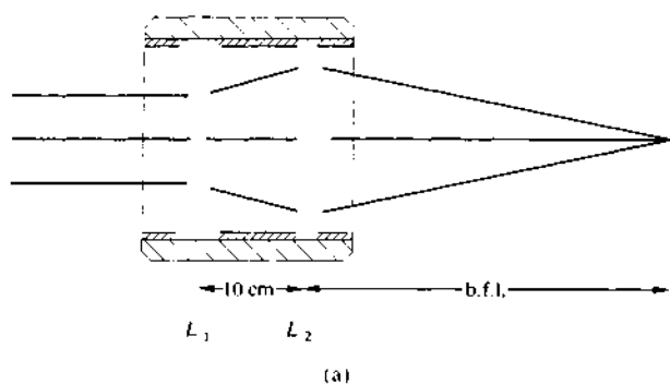
Figure 5.31 (a) A positive and negative thin-lens combination, (b) photo (Photo by E.H.I)
