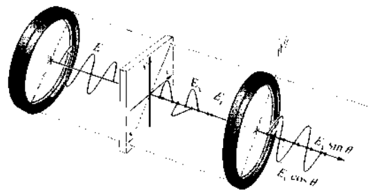
Figure 8.46 The origin of interference colors.
