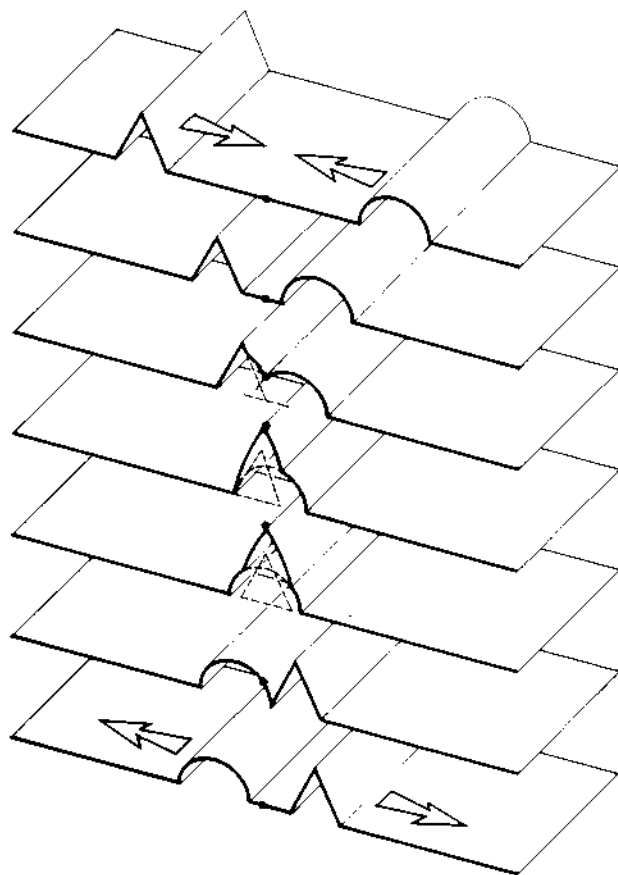
Figure 7.1 The superposition of two disturbances.
