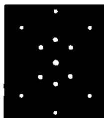
Diffraction pattern
