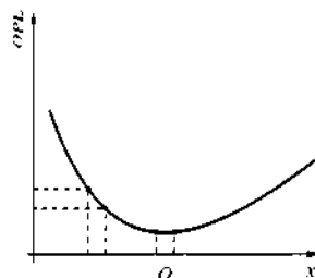
Figure 4.34 In the situation shown in Fig. 4.29 the actual location of point O corresponds to a path of minimum OPL.
