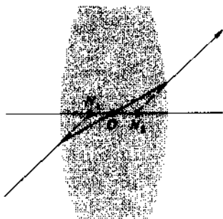
Figure 6.2 Nodal points.
