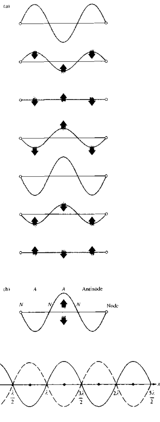
Figure 7.11 A standing wave at various times.
