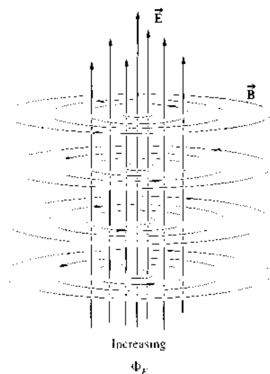
Figure 3.12 A time-varying \vec{E} -field. Surrounding each point where \Phi_E is changing, the \vec{B} -field forms closed loops.
