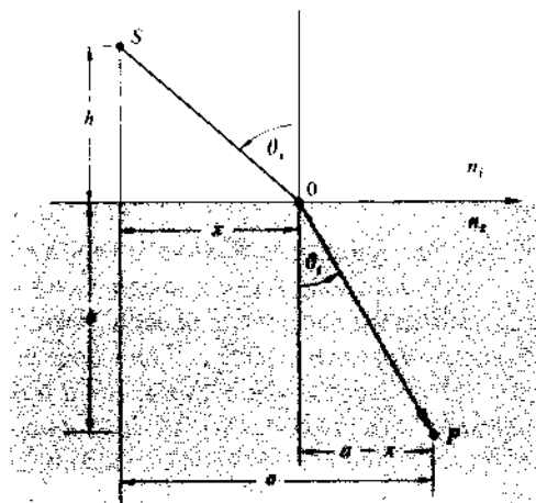
Figure 4.29 Fermat's Principle applied to refraction.
