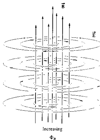
Figure 3.5 A time-varying \vec{B} -field. Surrounding each point where \Phi_M is changing, the \vec{E} -field forms closed loops.
