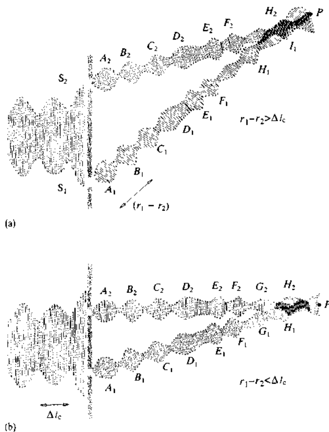
Figure 9.10 A schematic representation of how light, composed of a progression of wavegroups with a coherence length \Delta l_c , produces interference when (a) the path length difference exceeds \Delta l_c and (b) the path length difference is less than \Delta l_c .
