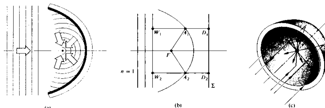
Figure 5.45 A paraboloidal mirror.
