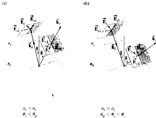
Figure 4.46 The reflected \vec{E} -field at various angles concomitant with internal reflection.
