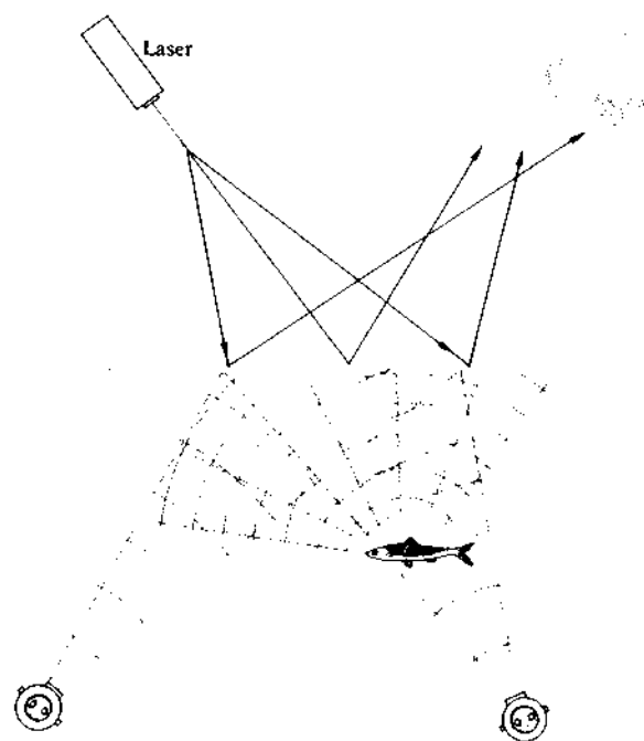
Figure 13.55 Acoustical holography.
