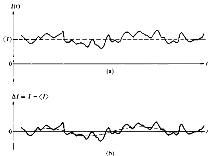
Figure 12.14 Irradiance variations.
