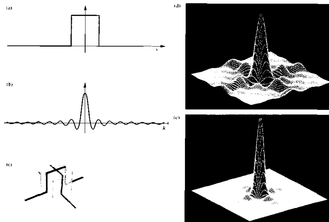
Figure 7.40 (a) A one-dimensional square pulse and (b) its transform. (c) A two-dimensional square pulse and (d) its transform. (e) The power spectrum of the transform in (d) plotted in two-dimensional k -space. (Photos courtesy R. G. Wilson, Illinois Wesleyan University.)
