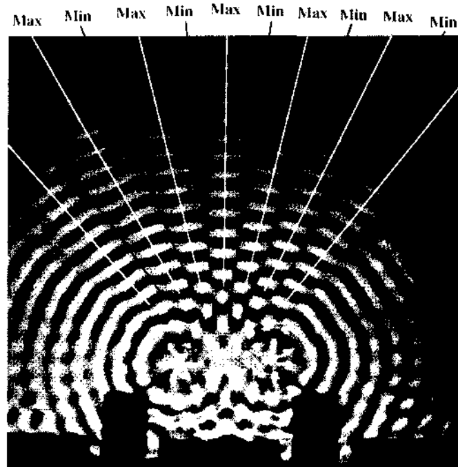
Figure 9.1 Water waves from two in-phase point sources in a ripple tank. In the middle of the pattern the wave peaks (thin bright bands), and troughs (thin black bands) lie within long wedge-shaped areas (maxima) separated by narrow dark regions of calm (minima). Although the nodal lines look straight, they're really hyperbolic. The optical equivalent is the electric field distribution depicted in Fig. 9.3c. (Photo courtesy PSSC College Physics, 1968, © 1965 Educational Development Center, Inc.)
