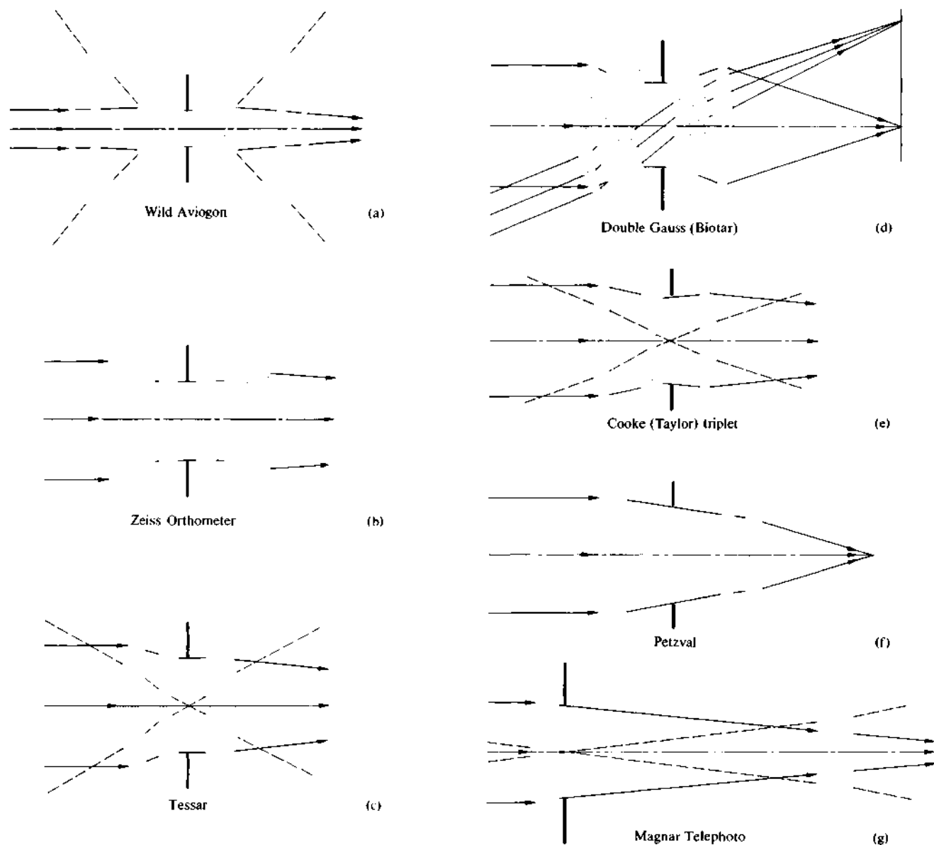
Figure 5.104 Camera lenses.
