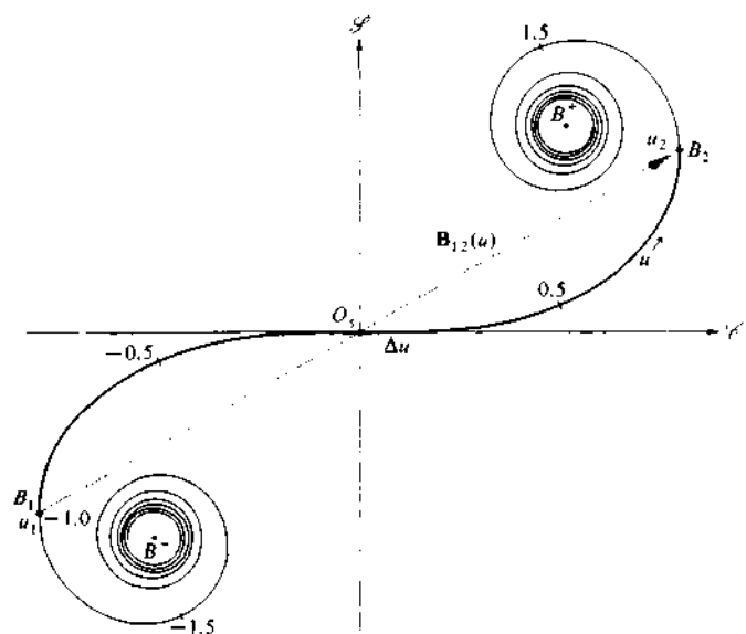
Figure 10.51 Cornu spiral.
