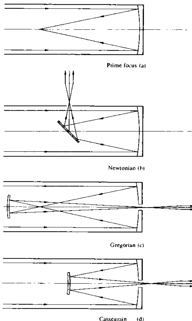
Figure 5.111 Reflecting telescopes.
