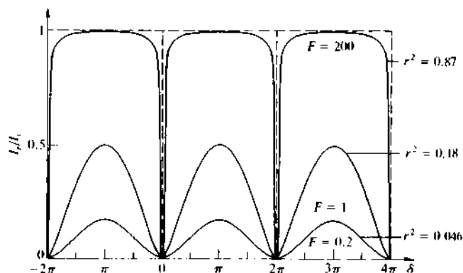
Figure 9.42 One minus the Airy function.
