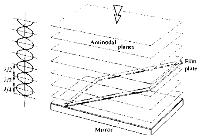
Figure 7.14 Wiener's experiment.
