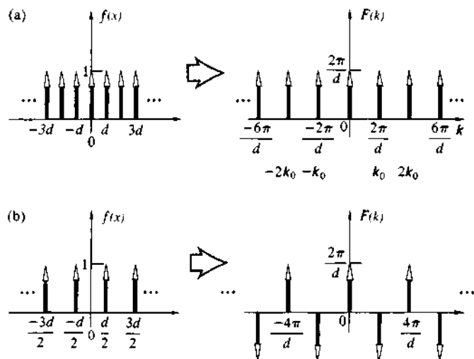
Figure 11.14 (a) The comb function and its transform. (b) A shifted comb function and its transform.
