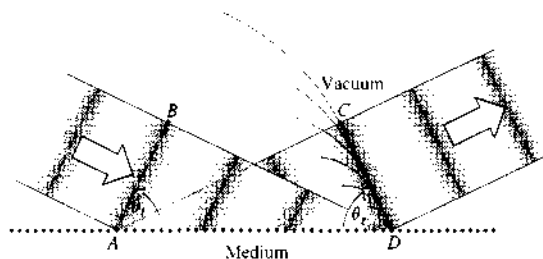
Figure 4.16 Plane waves enter from the left and are reflected off to the right. The reflected wavefront CD is formed of waves scattered by the atoms on the surface from A to D . Just as the first wavelet arrives at C from A , the atom at D emits, and the wavefront along CD is completed.
