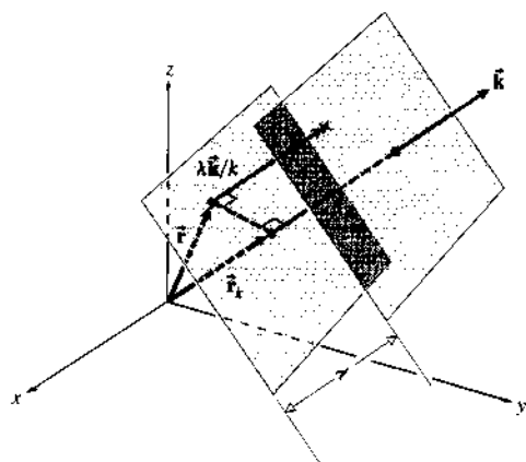
Figure 2.21 Plane waves.
