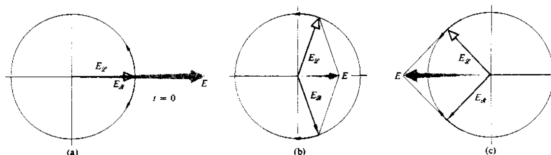
Figure 8.49 The superposition of an R - and an L -state at z = 0 .
