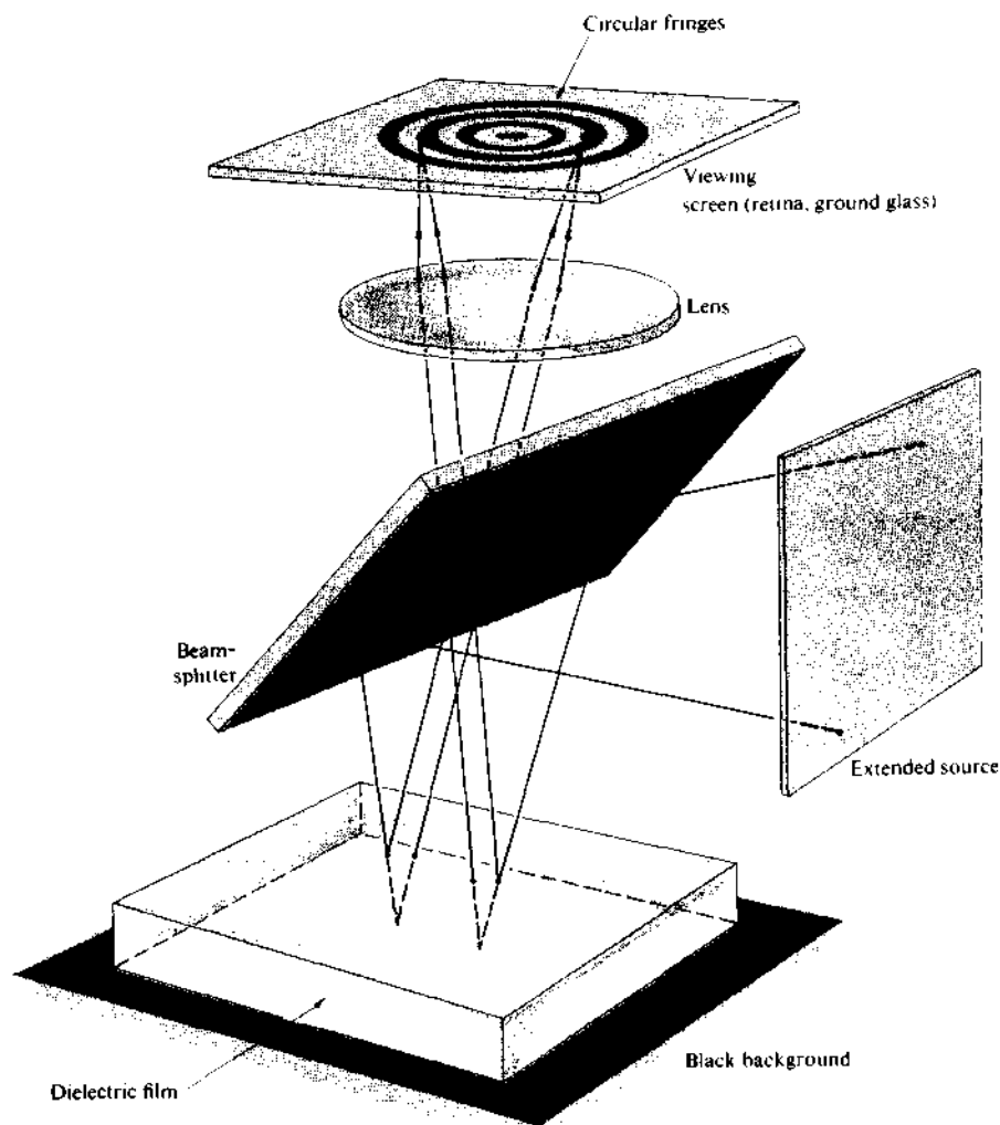
Figure 9.21 Circular Haidinger fringes centered on the lens axis.
