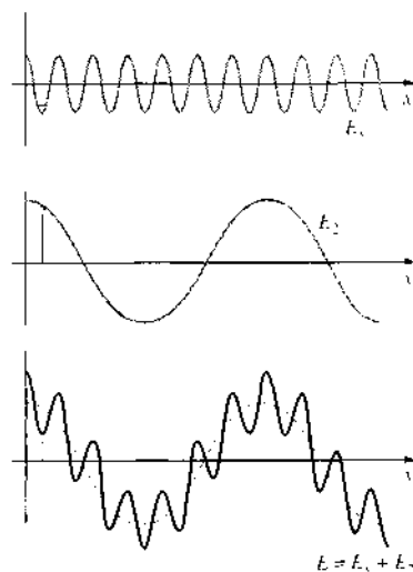
Figure 7.24 The superposition of two harmonic waves of different frequency produces a periodic anharmonic wave.
