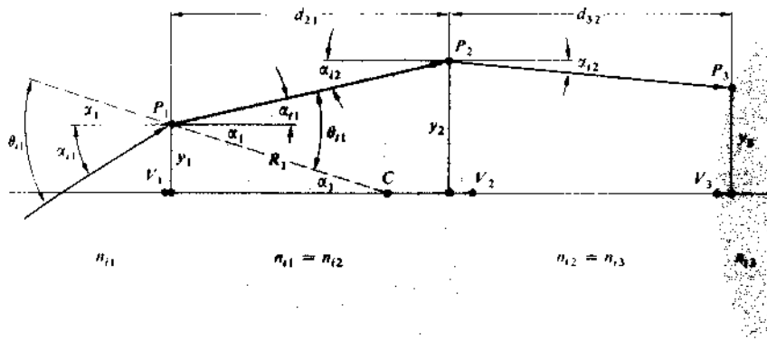
Figure 6.7 Ray geometry.
