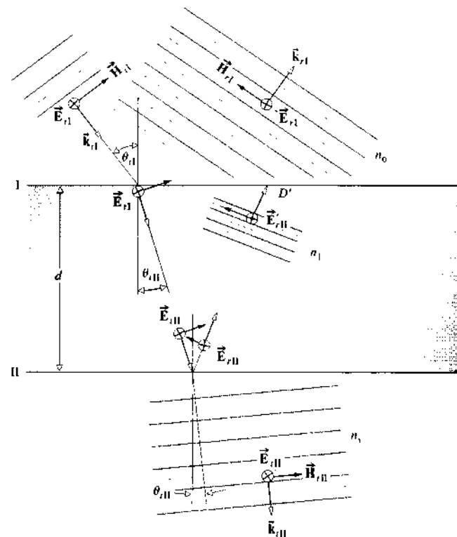
Figure 9.49 Fields at the boundaries.
