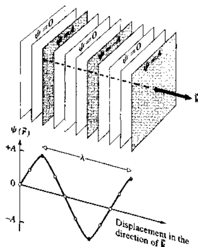
Figure 2.20 Wavefronts for a harmonic plane wave.
