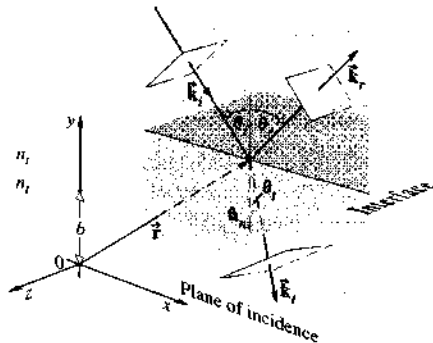
Figure 4.38 Plane waves incident on the boundary between two homogeneous, isotropic, lossless dielectric media.
