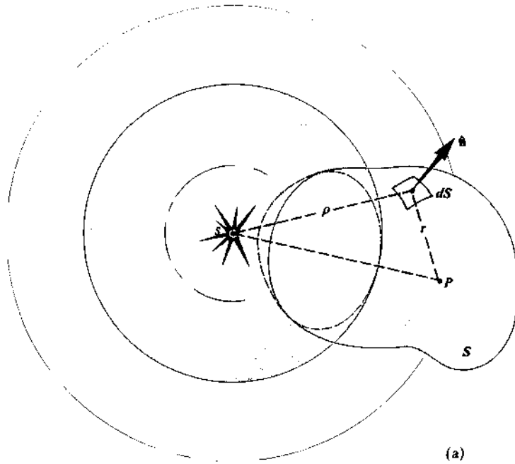
Figure 10.65 A spherical wave emitted from point s.
