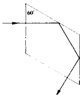
Figure 8.42 The Mooney rhomb.
