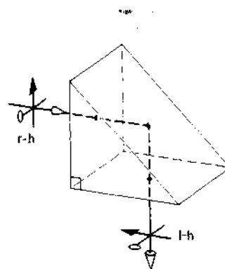
Figure 5.61 The right-angle prism.
