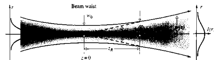
Figure 13.15 The spreading of a Gaussian beam.
