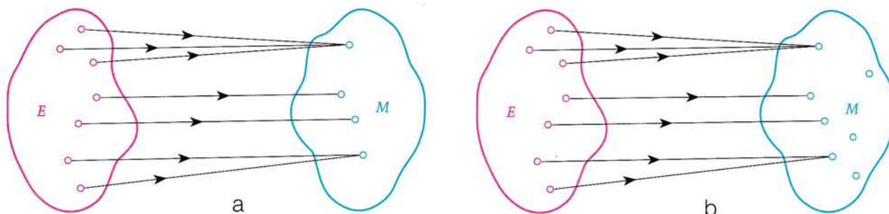
Figure 4 Mappings of (a) E onto M , (b) E into M .
