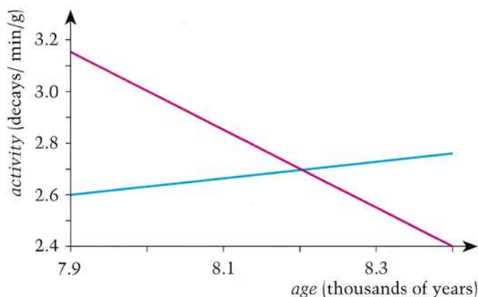
Figure 1 The age assuming a 1% decrease per century.
