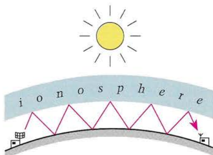
Figure 1 Two natural plasmatic objects and a schematic rendering of long-distance radio broadcasting.
