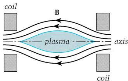
Figure 2 The mirror plasma trap.
