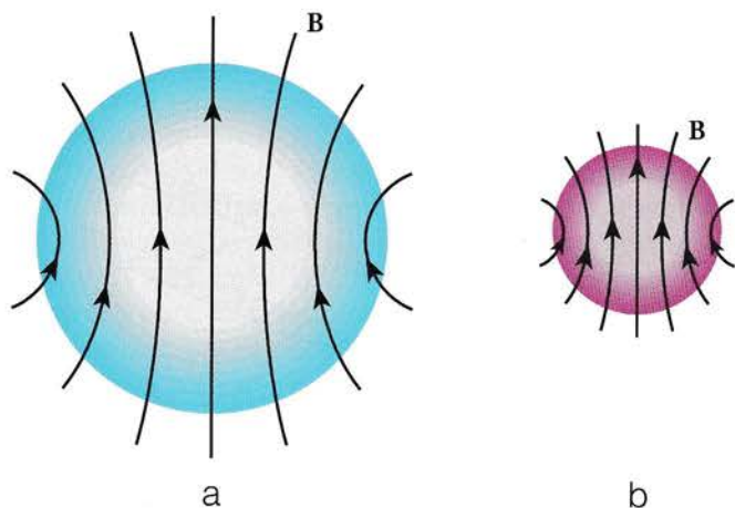
Figure 5 The "freezing-in" effect (a) in the initial state of a star; (b) in its final state (a neutron star).
