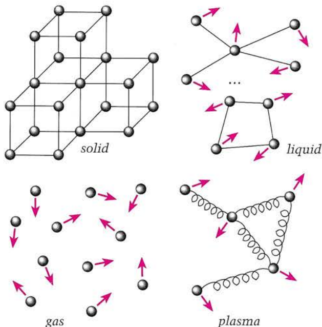
Figure 6 The four states of matter.
