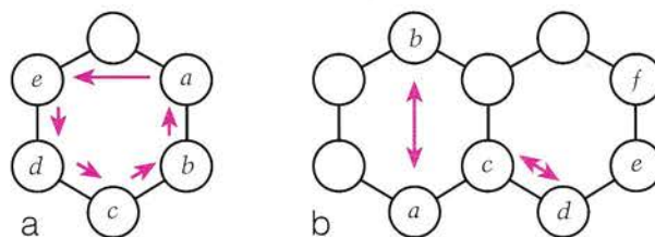
Figure 5 (a) Successively sliding chips a, b, c, d, e, a , we obtain their cyclic permutation, shown by the red arrows; (b) let L and R be the counterclockwise cyclic permutations of figure (a) for the left and right hexagons, respectively, L^{-1} and R^{-1} the inverse (clockwise) cycles, L^2 = LL and L^{-2} = L^{-1}L^{-1} the cycles L and L^{-1} repeated twice. Then the operation R^{-1}LRL^{-2}R^{-1}L^2RL^{-1} yields two simultaneous pair exchanges a \leftrightarrow b and c \leftrightarrow d .
