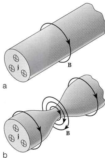
Figure 4 The pinch effect: (a) steady, (b) unstable.
