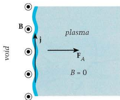
Figure 3 Magnetic confinement.
