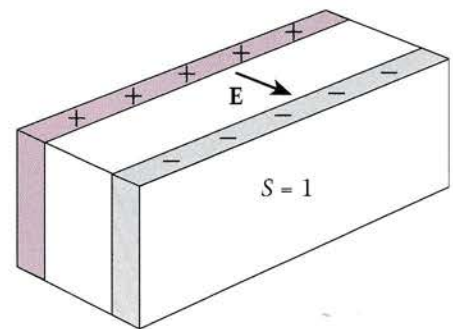
Figure 7 Deriving the Langmuir frequency.
